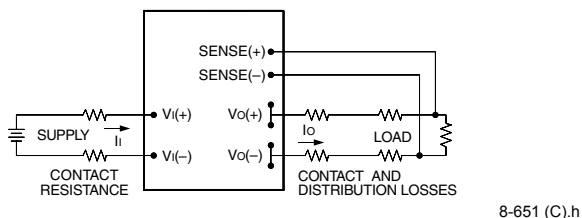
Figure 12. Effective Circuit Configuration for Single-Module Remote-Sense Operation
