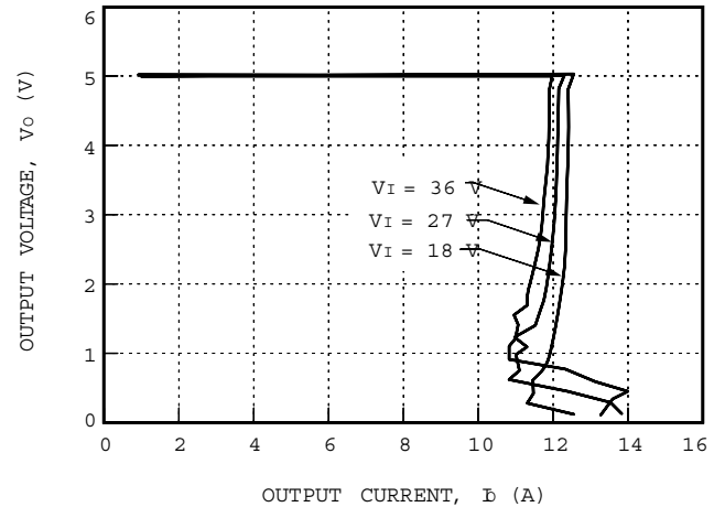
Figure 4. Typical JC050A Output Characteristics at Room Temperature
