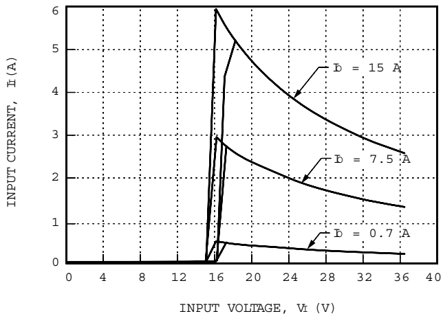
Figure 2. Typical JC075A Input Characteristics at Room Temperature
