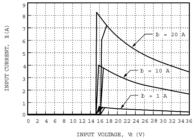
Figure 3. Typical JC100A Input Characteristics at Room Temperature
