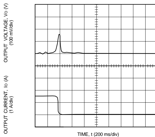
Figure 8. Typical JC100C Transient Response to Step Decrease in Load from 50% to 25% of Full Load at Room Temperature and 28 V Input (Waveform Averaged to Eliminate Ripple Component.)
