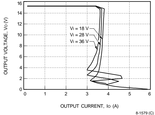
Figure 3. Typical JC050C Input Characteristics at Room Temperature
