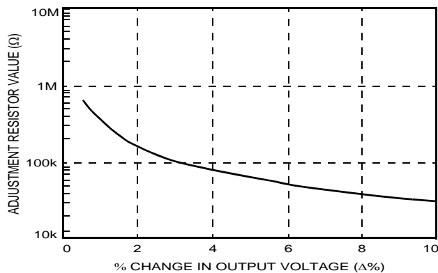
Figure 16. Resistor Selection for Increased Output Voltage
