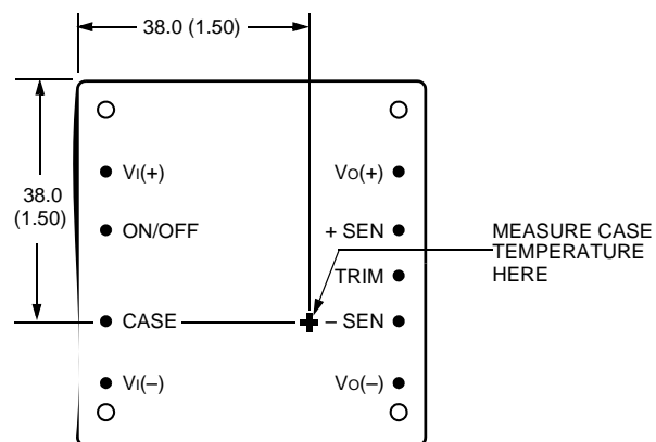
Figure 17. Case Temperature Measurement Location
