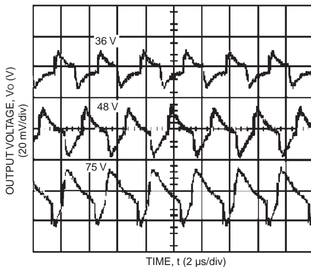
Figure 4. Typical Output Ripple Voltage at Room Temperature, Io = Full Load
