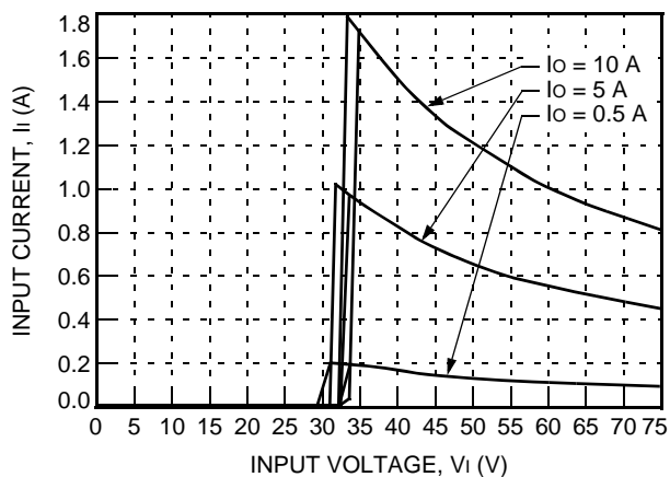
Figure 1. Typical JAW050A Input Characteristics at Room Temperature
