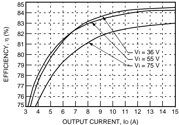
Figure 4. Typical JAW075A Efficiency vs. Output Current at Room Temperature
