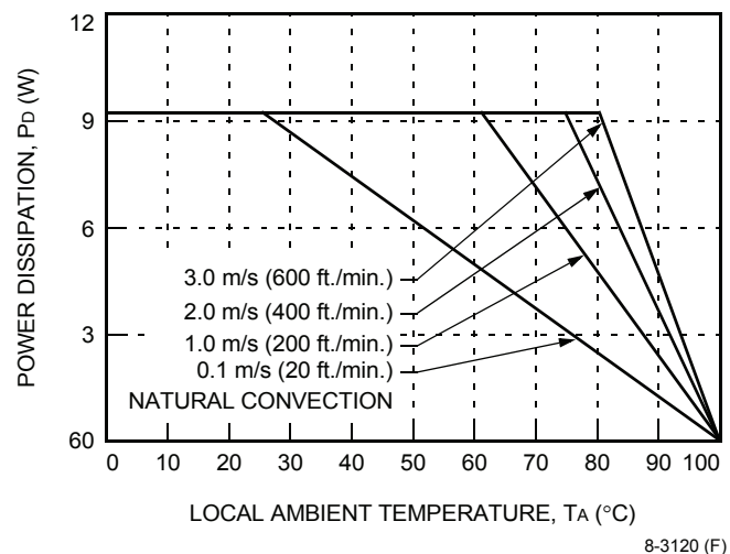
Figure 27. Forced Convection Power Derating with No Heat Sink; Either Orientation
