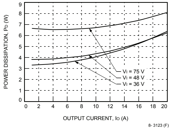
Figure 30. JAHW100G Power Dissipation vs. Output Current at 25 °C
