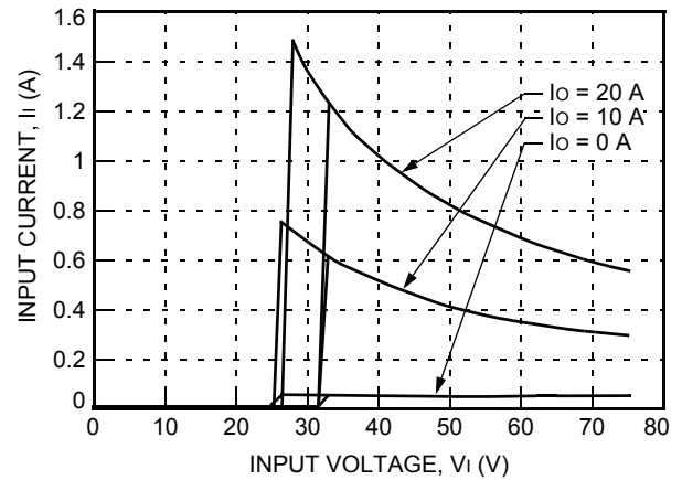
Figure 3. Typical JAHW100Y Input Characteristics at Room Temperature
