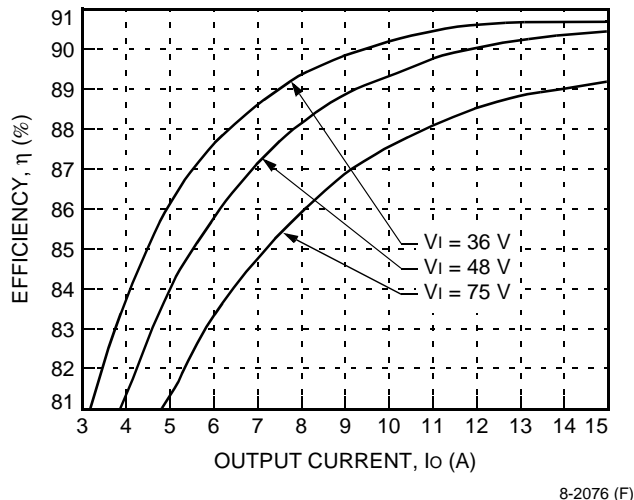
Figure 4. Typical JAHW075A Converter Efficiency vs. Output Current at Room Temperature
