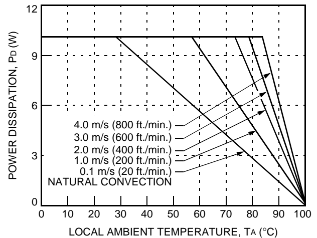
Figure 21. JAHW050A and JAHW075A Forced Convection Power Derating with No Heat Sink; Either Orientation
