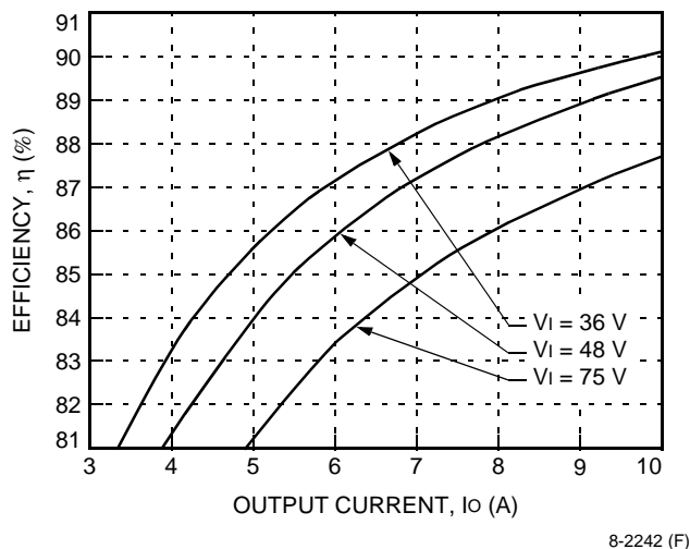
Figure 3. Typical JAHW050A Converter Efficiency vs. Output Current at Room Temperature
