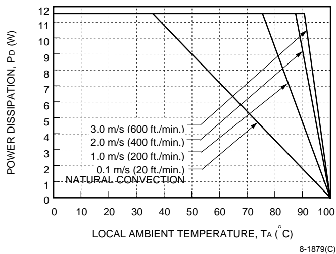
Figure 25. HW100A1 Power Derating vs. Local Ambient Temperature and Air Velocity; Best Orientation
