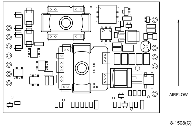
Figure 18. Best Orientation (Top View)
