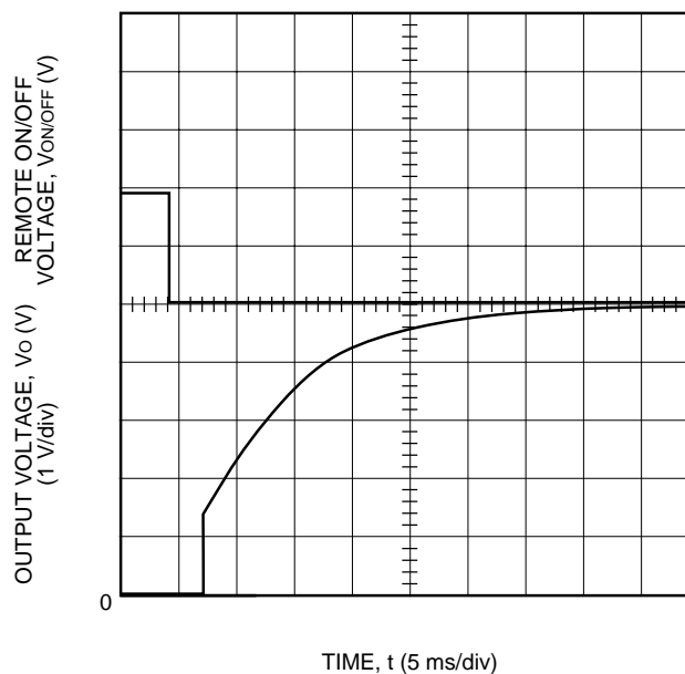
Figure 7. Typical Start-Up from Remote On/Off HW100A1; I_o = I_{o, \max}
