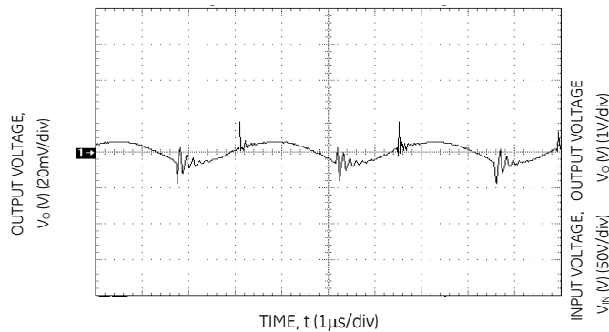
Figure 8. Typical Output Ripple and Noise.
