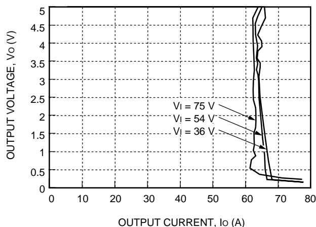
Figure 4. Typical FW300A1 Output Characteristics at Room Temperature
