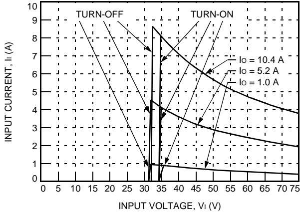
Figure 1. Typical FW250H1 Input Characteristics at Room Temperature
