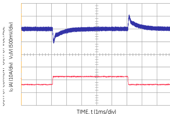
Figure 3. Transient Response to Dynamic Load Change from 25% to 50% to 25% of Full Load at Room Temperature and 48 Vdc Input; 0.1A/μs ; C_{o,ext} = 470\mu\text{F} .
