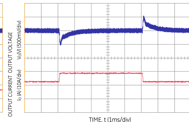
Figure 6. Transient Response to Dynamic Load Change from 50% to 75% to 50% of Full Load at Room Temperature and 48 Vdc Input; 0.1A/μs ; C_{o,ext} = 470\mu\text{F} .
