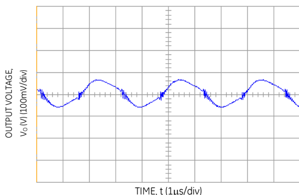
Figure 2. Typical Output Ripple and Noise at Room Temperature and 48Vin; I_o = I_{o,max} ; C_{o,ext} = 470\mu\text{F} .
