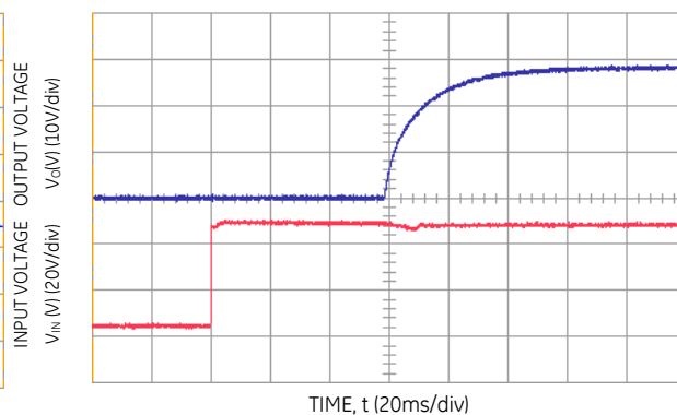
Figure 5. Typical Start-Up Using from V_{IN} , positive logic version shown; C_{o,ext} = 470\mu\text{F} .
