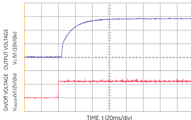
Figure 4. Typical Start-Up Using Remote On/Off, R1=30\text{Kohm} ; C_{o,ext} = 470\mu\text{F} .
