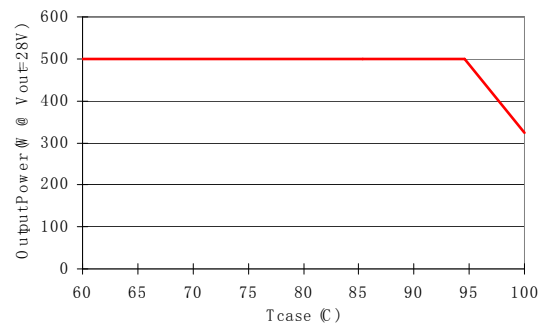
Figure 15. Output Power Derating for FNW500R in Conduction cooling (cold plate) applications; T_a < 72^\circ\text{C} in vicinity of module interior; V_{IN} = V_{IN, NOM}
