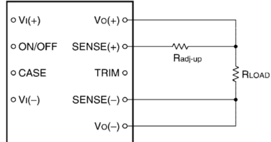
Figure 12. Circuit Configuration to Increase Output Voltage.
