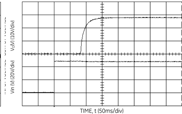
Figure 5. Typical Start-Up Using from V_{IN} , positive logic version shown; C_{o,ext} = 470\mu F .
