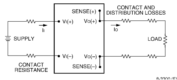
Figure 9. Output Voltage and Efficiency Test Setup.
