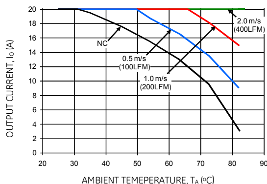
Figure 17. Output Current Derating for the Module with Heatplate; Airflow in the Transverse Direction from V_{out}(+) to V_{out}(-) ; V_{in} = 48\text{V} .
