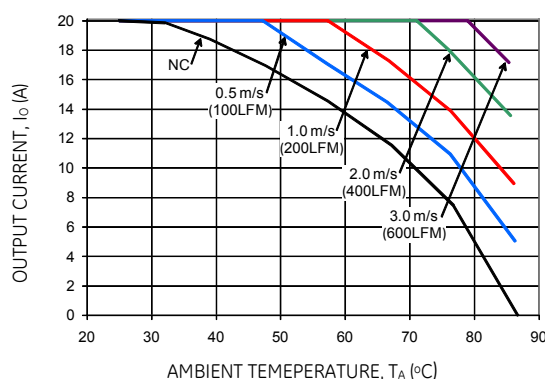
Figure 16. Output Current Derating for the Open Frame Module; Airflow in the Transverse Direction from V_{out}(+) to V_{out}(-) ; V_{in} = 48\text{V} .
