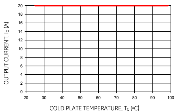
Figure 15. Output Current Derating for the Module in Conduction Cooling (cold plate) Applications, with or without Heatplate; T_a < 70^\circ\text{C} in vicinity of module interior; V_{in} = 48\text{V} .
