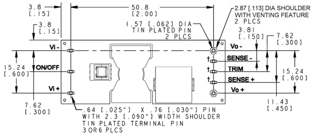
Bottom View
