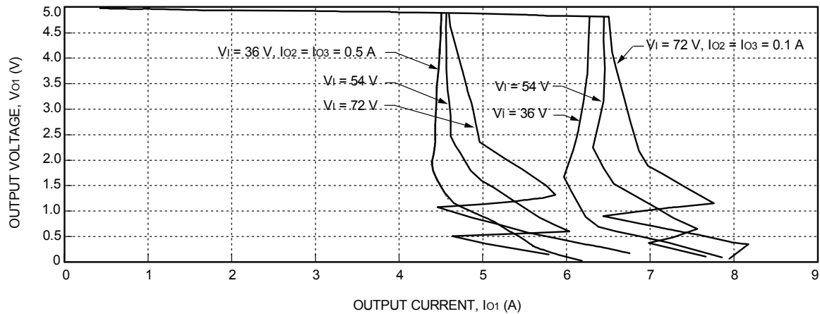
Figure 9. DW025ABK-M Typical 5 V Output Characteristics
