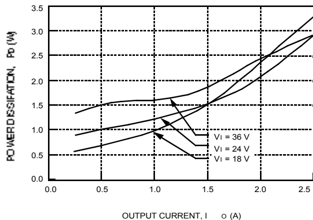
Figure 16. 3.3 V Output Power Dissipation vs. Output Current
