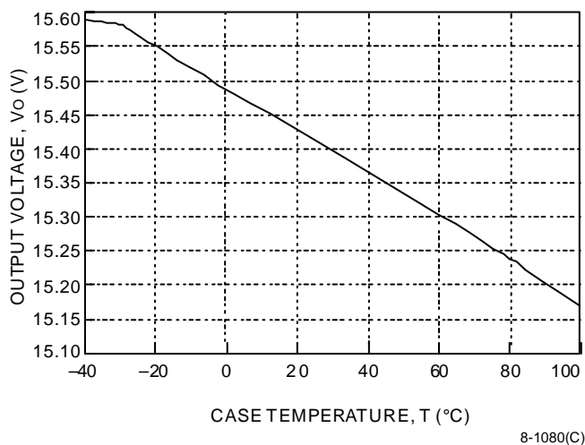
Figure 4. DC025 Triple Output-Series Typical Output Voltage Variation of 15 V Output Over Ambient Temperature Range
