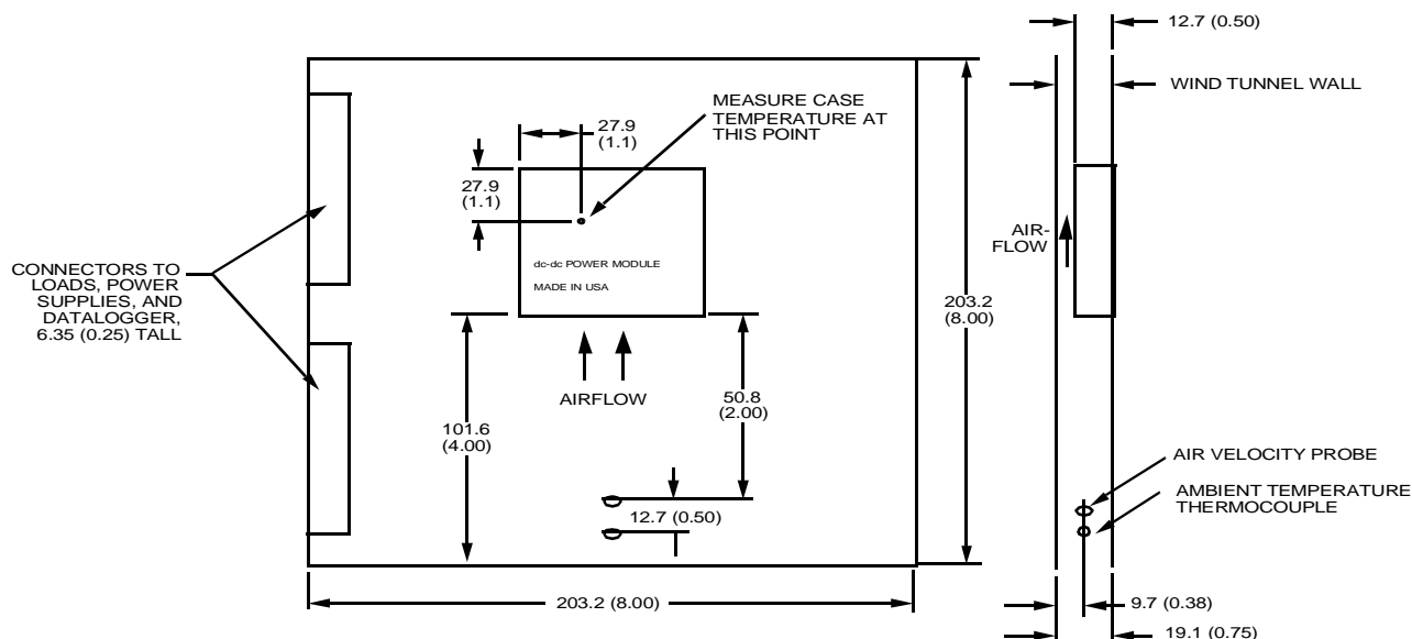
Figure 22. Thermal Test Setup
