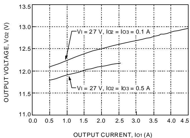
Figure 6. DC025ABK-M Typical Cross Regulation with Respect to I_{o1}
