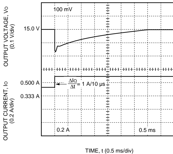
Figure 9. CW025 Dual Output-Series Typical 15 V Output Voltage Response to a Step Load Change from 50% to 75% of I_{o,max} at V_i = V_{i,nom} and T_c = 25\text{ }^{\circ}\text{C}
