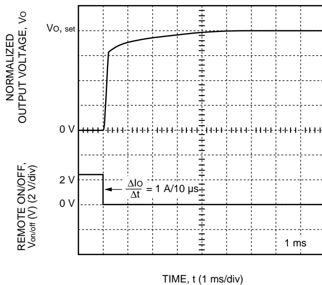
Figure 10. CW025 Dual Output-Series Typical Output Voltage Rise Time with Remote On/Off at V_i = V_{i,nom} , I_o = 0.8 (I_{o,max}) and T_c = 25\text{ }^{\circ}\text{C}
