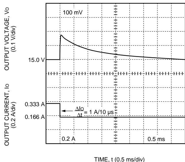
Figure 6. CW025 Dual Output-Series Typical 15 V Output Voltage Response to a Step Load Change from 50% to 25% of I_{o,max} at V_i = V_{i,nom} and T_c = 25\text{ }^{\circ}\text{C}
