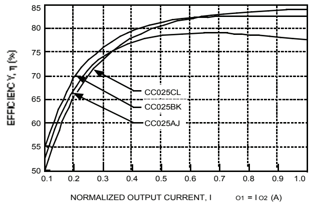
Figure 3. CC025 Dual-Output-Series Efficiency vs. Normalized Output Currents at V_i = 28\text{ V} and T_c = 25^\circ\text{C}
