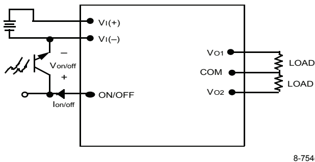
Figure 14. Remote On/Off Implementation
