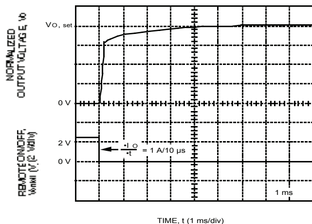
Figure 10. CC025 Dual-Output-Series Typical Output Voltage Rise Time with Remote On/Off at V_i = V_{i,nom} , I_o = 0.8 (I_{o,max}) , and T_c = 25^\circ\text{C}
