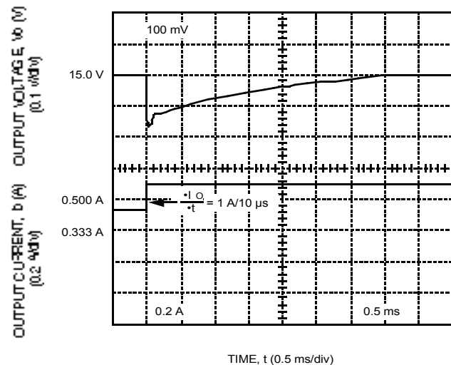
Figure 9. CC025 Dual-Output-Series Typical 15 V Output Voltage Response to a Step Load Change from 50% to 75% of I_{o,max} at V_i = V_{i,nom} and T_c = 25^\circ\text{C}
