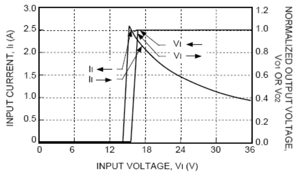
Figure 1. CC025 Dual-Output-Series Input Current and Normalized Output Voltage vs. Input Voltage at Full Load and T_c = 25^\circ\text{C}
