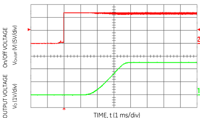
Figure 15. Typical Start-Up Using Remote On/Off with Low-ESR external capacitors ( C_o = 5000\text{ }\mu\text{F} ) ( V_{in} = 12.0\text{ Vdc} , V_o = 5.0\text{ Vdc} , I_o = 10.0\text{ A} , C_o = 1050\text{ }\mu\text{F} ).
