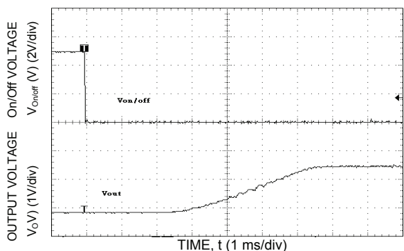
Figure 15. Typical Start-Up Using Remote On/Off with Low-ESR external capacitors (7x150µF Polymer) ( V_{in} = 12 Vdc, V_o = 3.3 Vdc, I_o = 5.0 A, C_o = 1050 µF).
