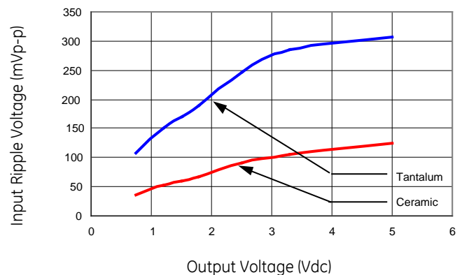
Figure 26. Input ripple voltage for various output with 2x47 \mu F tantalum capacitors and with 2x22 \mu F ceramic capacitors at the input (100% of I_{O,max} ).
