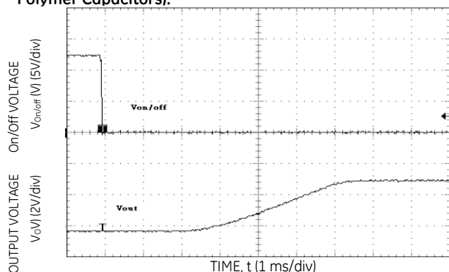
Figure 14. Typical Start-Up Using Remote On/Off ( V_{in} = 12 Vdc, V_o = 3.3 Vdc, I_o = 5.0 A).
