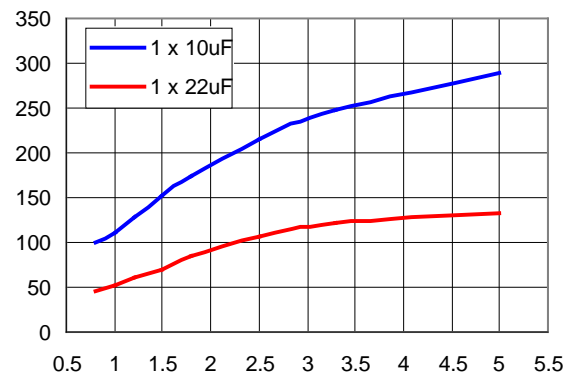
Figure 26. Input ripple voltage for various outputs with a 10 μF or a 22 μF ceramic capacitor at the input (full-load).
