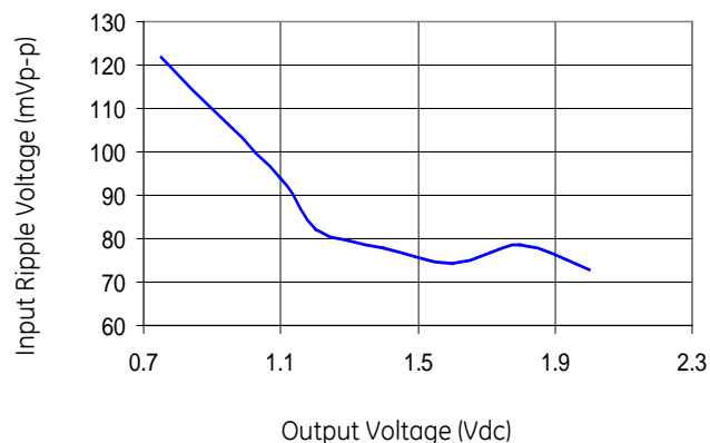
Figure 18. Input ripple voltage for various output with 2x150 \mu F polymer and 2x47 \mu F ceramic capacitors at the input ( V_{in}=3.3V , full load)
