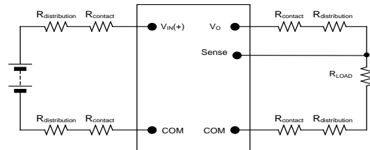
Figure 30. Remote sense circuit configuration
