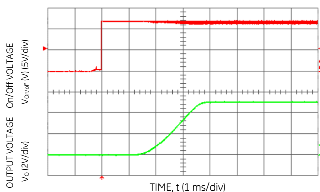
Figure 15. Typical Start-Up Using Remote On/Off with Low-ESR external capacitors ( C_o = 5000 \mu F) ( V_{in} = 12.0 Vdc, V_o = 5.0 Vdc, I_o = 10.0 A, C_o = 1050 \mu F).
