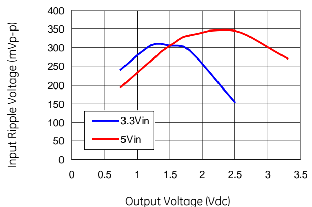
Figure 26. Input ripple voltage for various output with 1x150 \mu F polymer and 1x47 \mu F ceramic capacitors at the input (full load).
