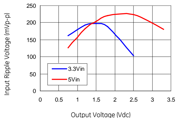
Figure 27. Input ripple voltage for various output with 2x150 \mu F polymer and 2x47 \mu F ceramic capacitors at the input (full load).
