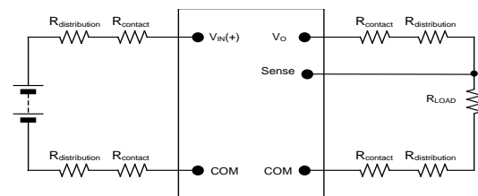
Figure 33. Remote sense circuit configuration.
