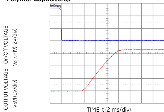
Figure 14. Typical Start-Up Using Remote On/Off ( V_{in} = 5.5 Vdc, V_o = 3.3 Vdc, I_o = 10 A).
