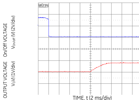
Figure 17. Typical Start-Up with Prebias ( V_{in} = 3.3 Vdc, V_o = 1.8 Vdc, I_o = 1 A, V_{bias} = 1.0 Vdc).
