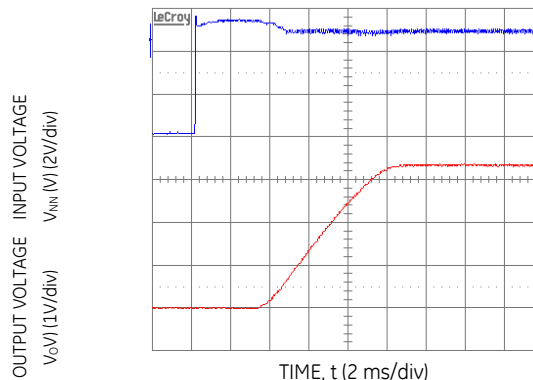
Figure 16. Typical Start-Up with application of V_{in} ( V_{in} = 5.5 Vdc, V_o = 3.3 Vdc, I_o = 10 A).
