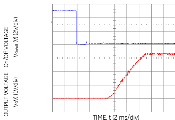
Figure 15. Typical Start-Up Using Remote On/Off with Low-ESR external capacitors (7x150uF Polymer) ( V_{in} = 5.0\text{Vdc} , V_o = 3.3\text{Vdc} , I_o = 6\text{A} , C_o = 1050\mu\text{F} ).
