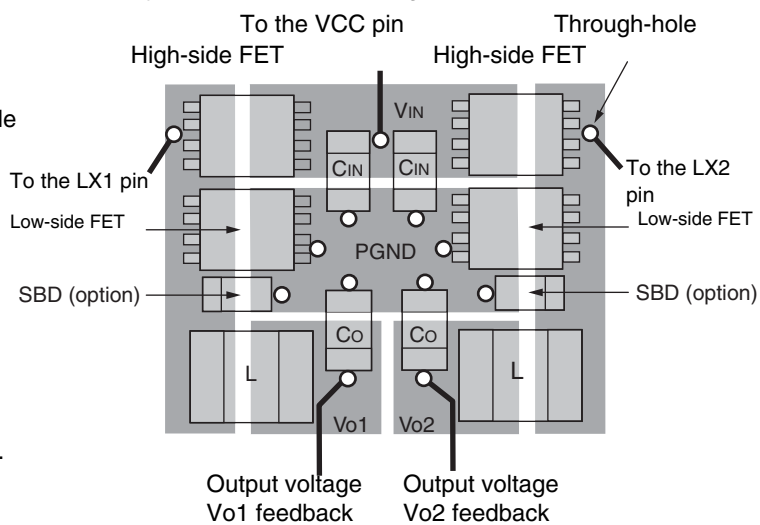
Layout example of switching components
