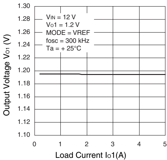
CH1 Load Regulation
