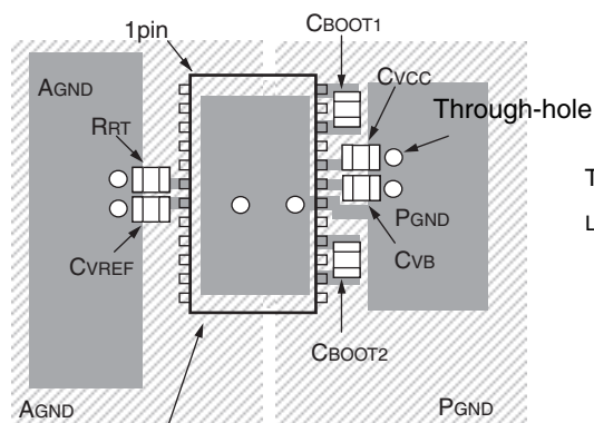
Layout example of IC
