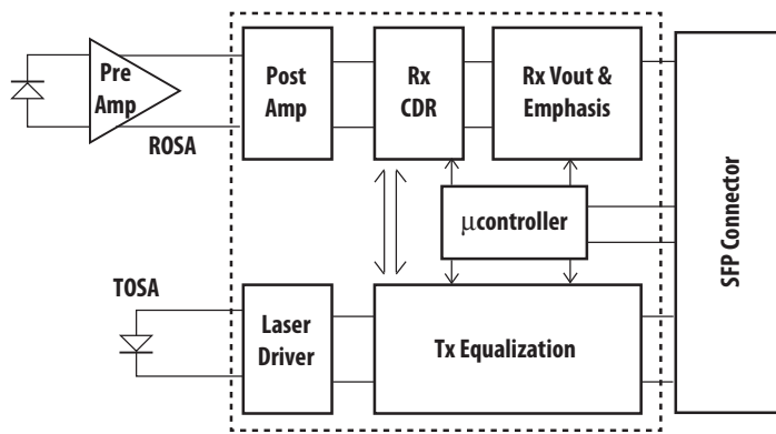
Figure 1. Transceiver functional diagram
