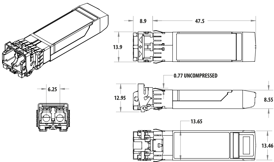
Figure 6. Module drawing
