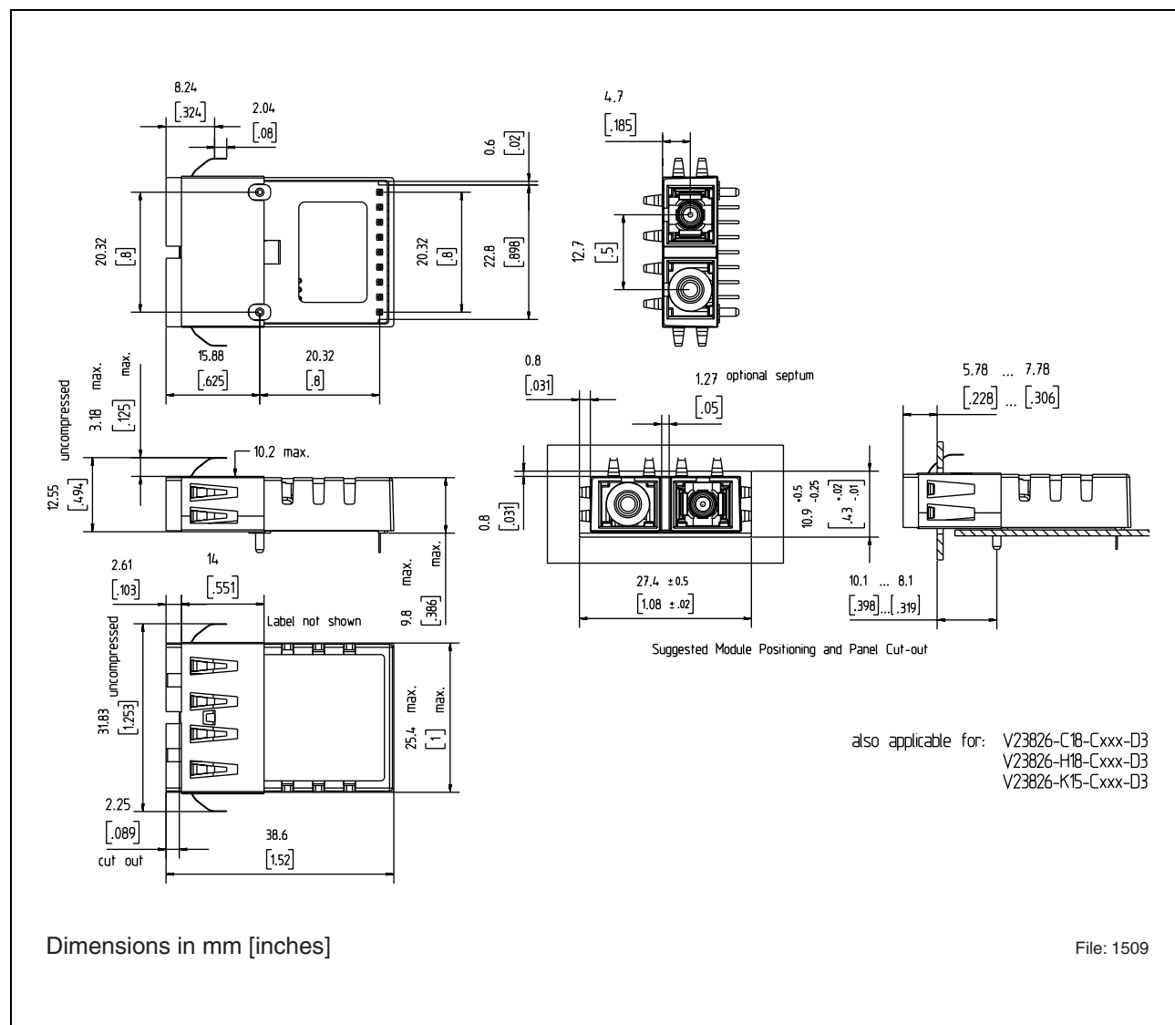
Figure 10 -D3 Shield with Backward Springs
