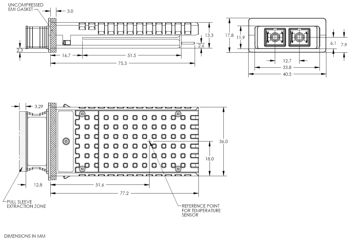
Figure 3-X2 Mechanical Dimensions
