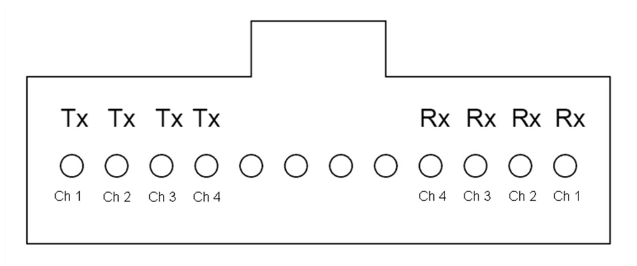
Figure 4 – FTL4P1QM1C optical lane assignment (front view of MPO receptacle)
