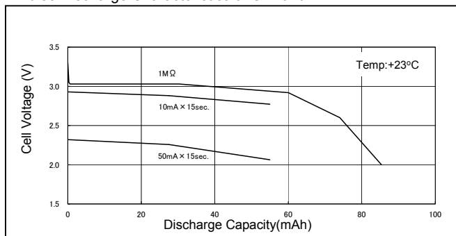
Pulse Discharge Characteristics of CR2016
