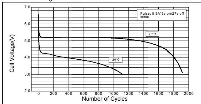
Pulse Discharge Characteristics of CR-P2
