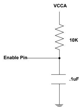
Fig. 19: RC Delay for Enable taken from VCCA
