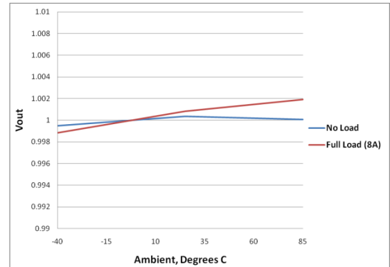
Fig. 16: XRP7708 Temperature Regulation 1.0V out (+/- 1% Vo window)
