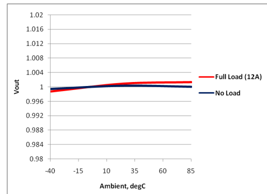
Fig. 188: XRP7740 Temperature Regulation 1.0V out (+/- 1% Vo window)
