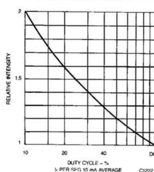
Fig. 4. Luminous Intensity vs. Duty Cycle
