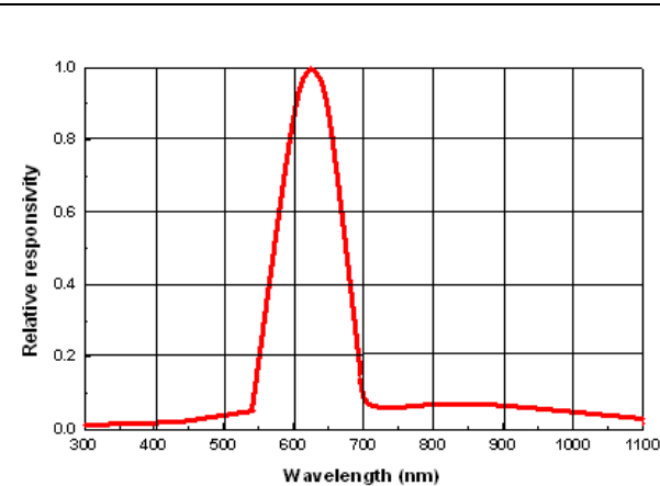
Fig.3 Spectral Response
