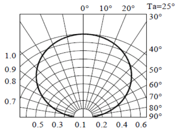
Radiation Diagram
