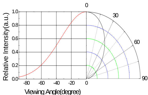
Radiation Characteristics
