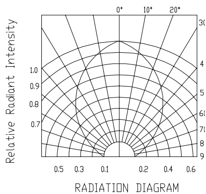
Radiation Diagram T_a=25^\circ C
