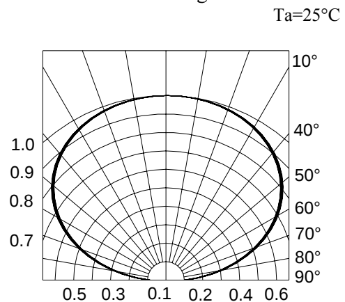
Radiation Diagram
