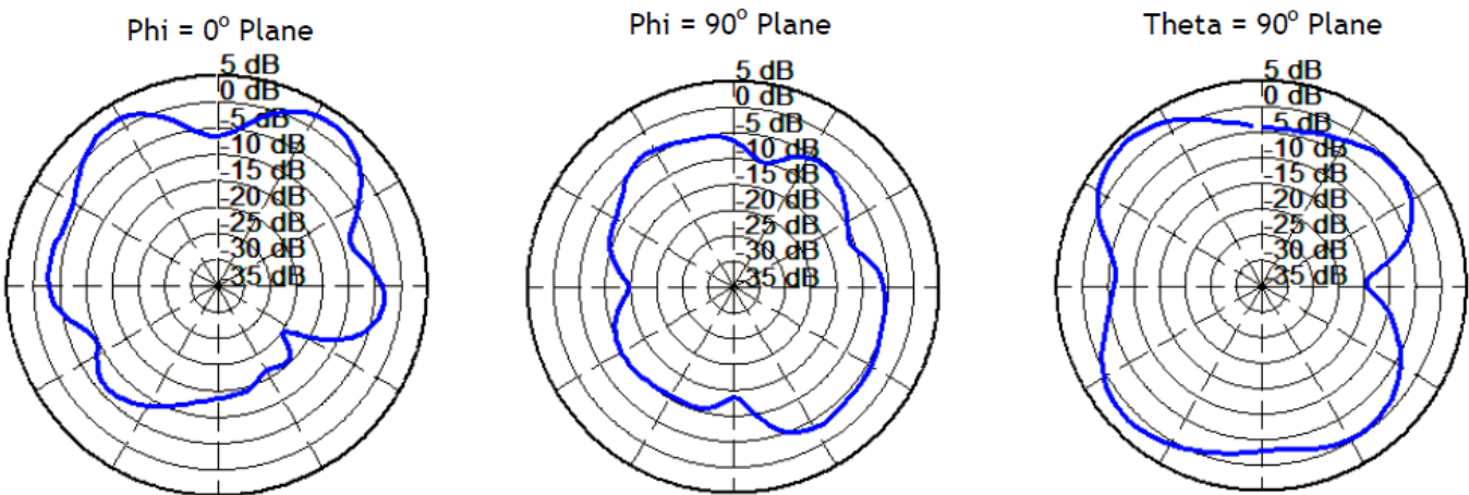
Measured at 5.1 GHz WLAN a
