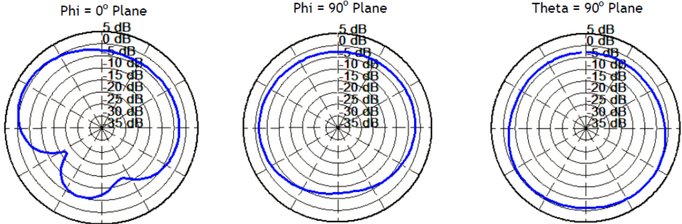
Measured at 5.1 GHz WLAN a
