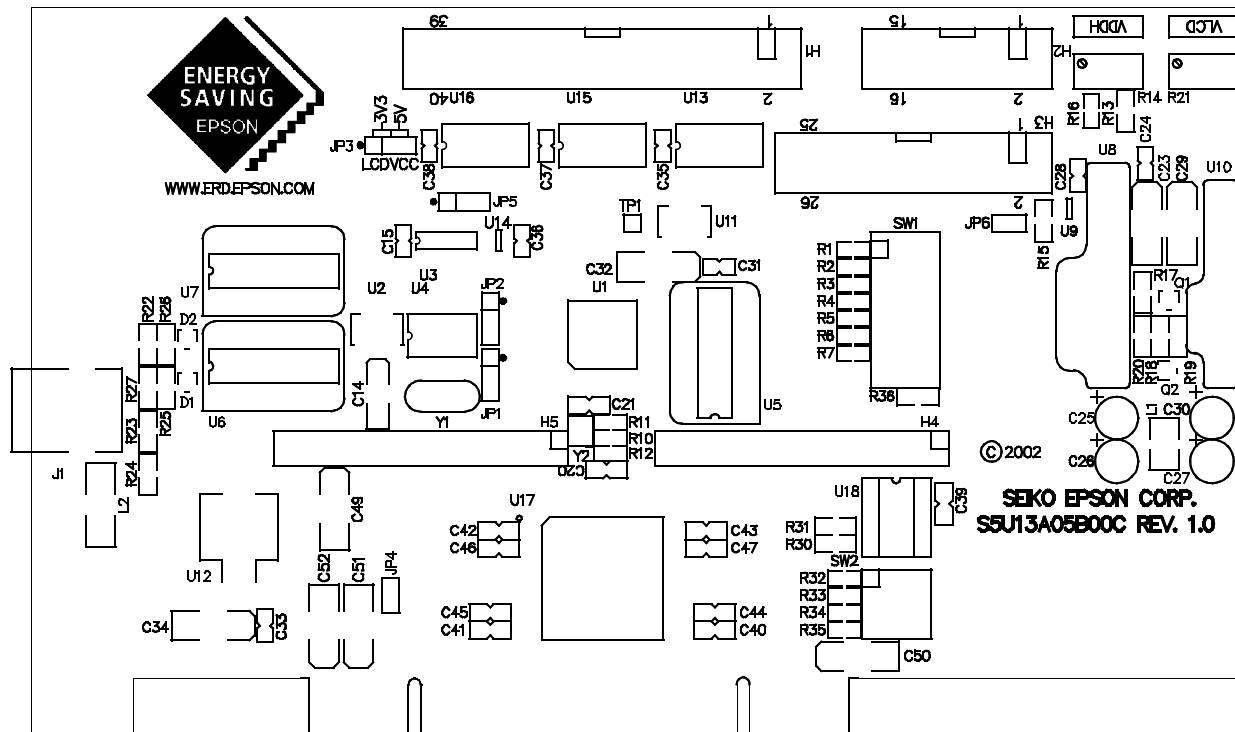
Figure 10-1: S5U13A05P00C100 Board Layout (Top View)
