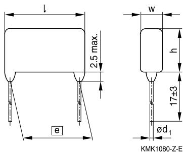
Straight leads
