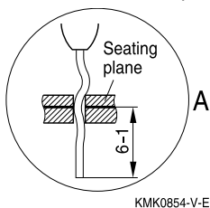
Detail of double crimped version
