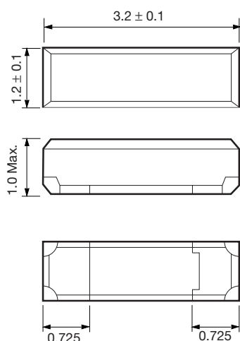
Figure 1) ECX-32 - Top, Side Bottom & End views
